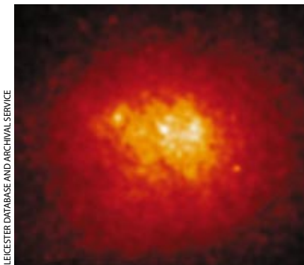
COMA CLUSTER looks different in visible light ( left ) and in x-rays ( right ). In visible light, it appears to be just an assemblage of galaxies. But in x-rays, it is a gargantuan ball of hot gas some five million light-years across.
