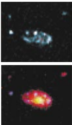
NASA AND ROGER L. THOMPSON/University of Arizona
